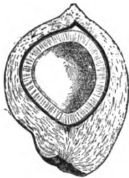
FIG. 260. — The Coconut, in section; reduced.
